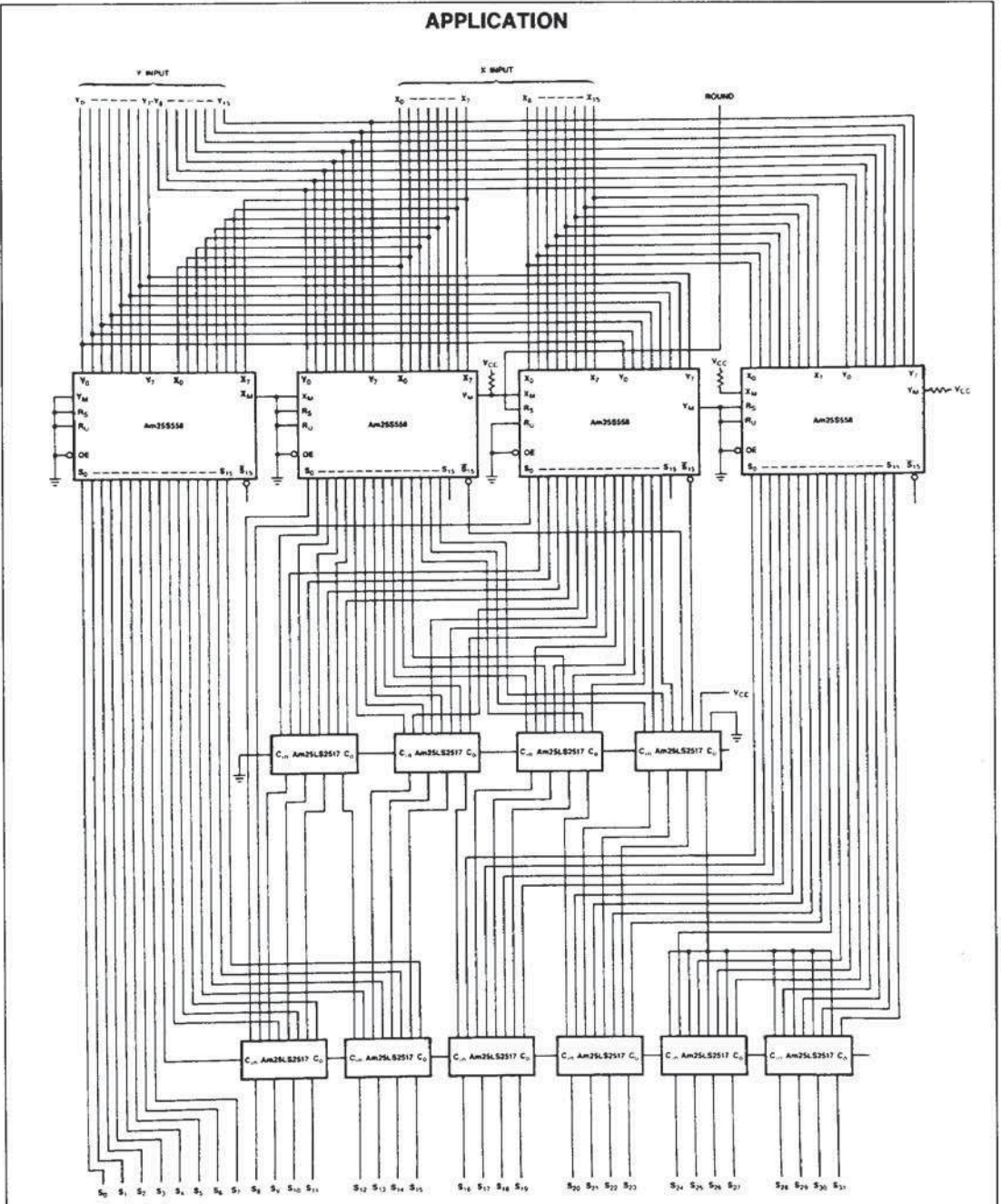
Figure 1. High-Speed 16 x 16 2's Complement Multiplication.
