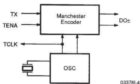
Figure 1. Transmit Section
