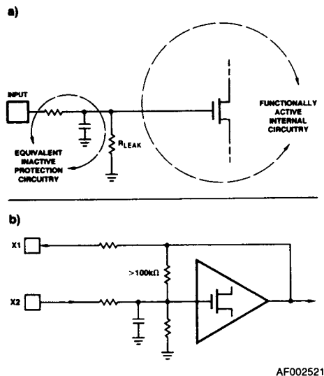
Figure 3. Input Circuitry
