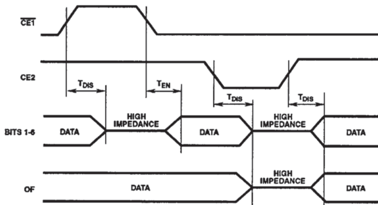
FIGURE 2. OUTPUT ENABLE
