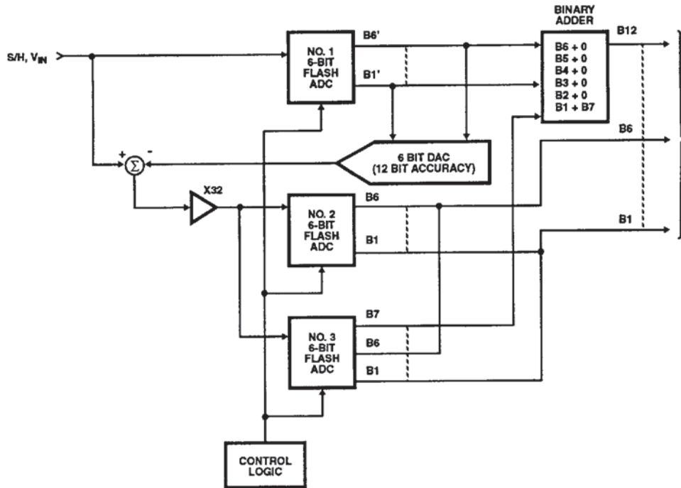
FIGURE 19. TYPICAL CA3306, 800ns, 12-BIT ADC SYSTEM
