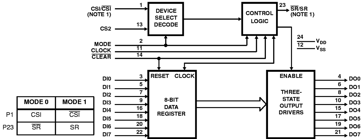
FIGURE 2. FUNCTIONAL BLOCK DIAGRAM FOR CDP1852
