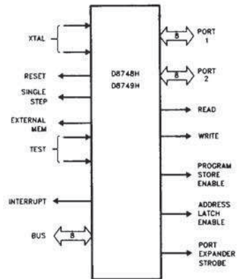
Figure 2. Logic Symbol
