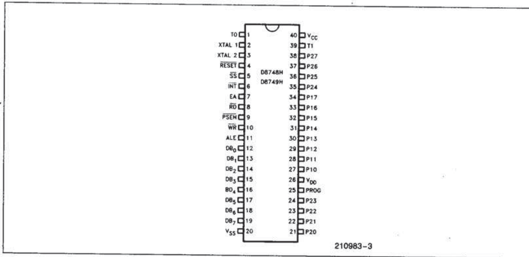
Figure 3. Pin Configuration
