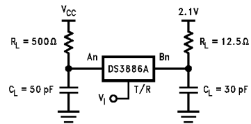
FIGURE 10. T/R to An, T/R to Bn
