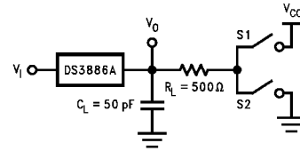
FIGURE 7. Receiver Enable/Disable Set-up
