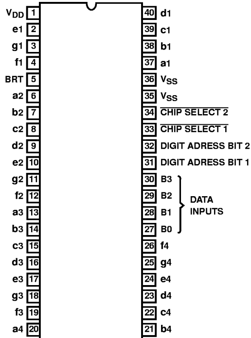
ICM7212AM (PDIP) TOP VIEW
