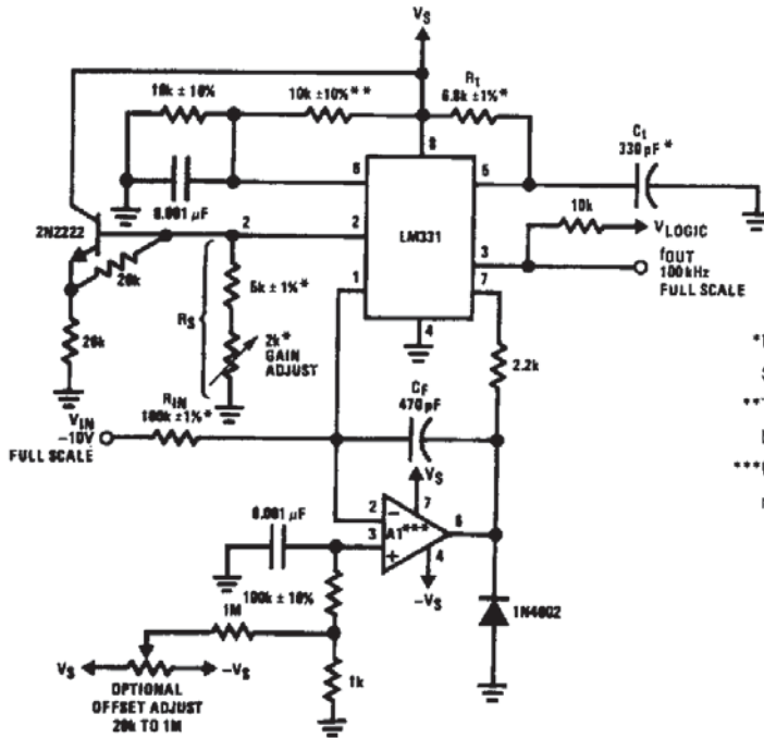
FIGURE 4. Precision Voltage-to-Frequency Converter, 100 kHz Full-Scale, ±0.03% Non-Linearity
