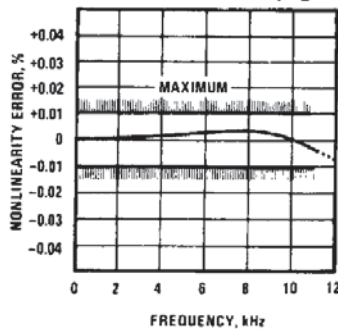
Nonlinearity Error, Precision F-to-V Converter (Figure 6)
