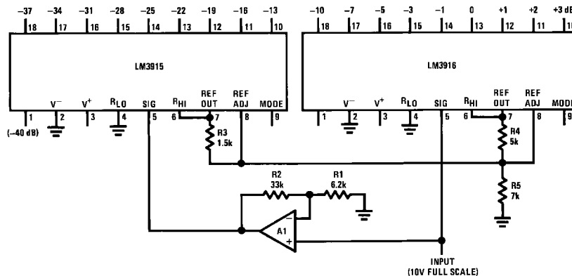
FIGURE 8. Low Cost Circuit for 40 dB Display
