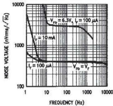
Reference Noise Voltage vs Frequency
