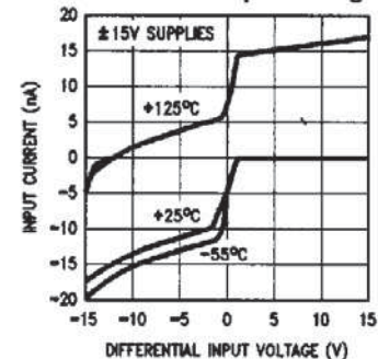
Input Current vs Differential Input Voltage
