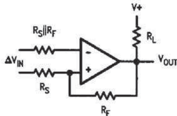
FIGURE 12. R_S and R_F Add Hysteresis to Comparator
