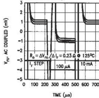
Reference Step Response for 100 µ ~ 10 mA Current Step
