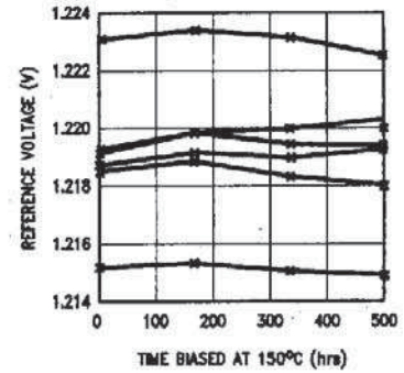
Accelerated Reference Voltage Drift vs Time
