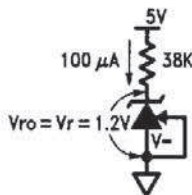
FIGURE 3. 1.2V Reference
