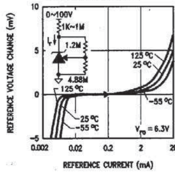
Reference Voltage vs Current and Temperature
