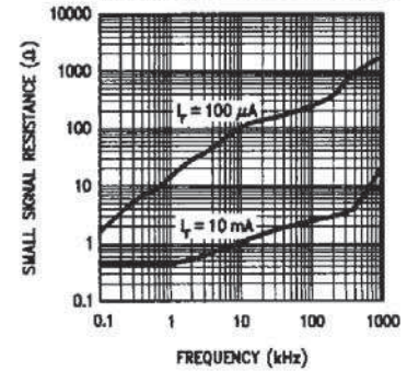
Reference Small-Signal Resistance vs Frequency
