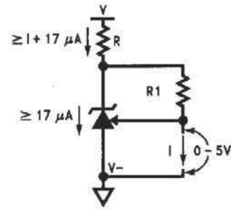
FIGURE 9. Current Source is Programmed by R1
