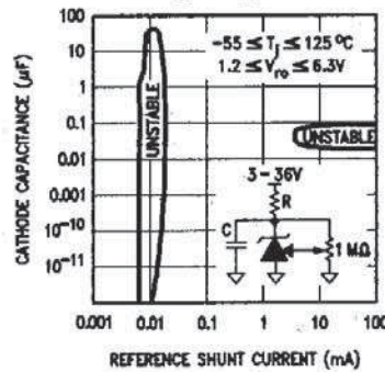
Reference AC Stability Range
