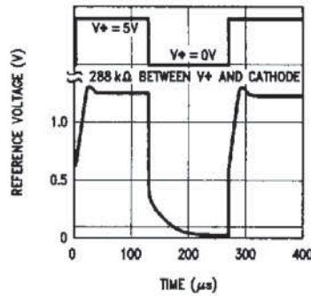
Reference Power-Up Time
