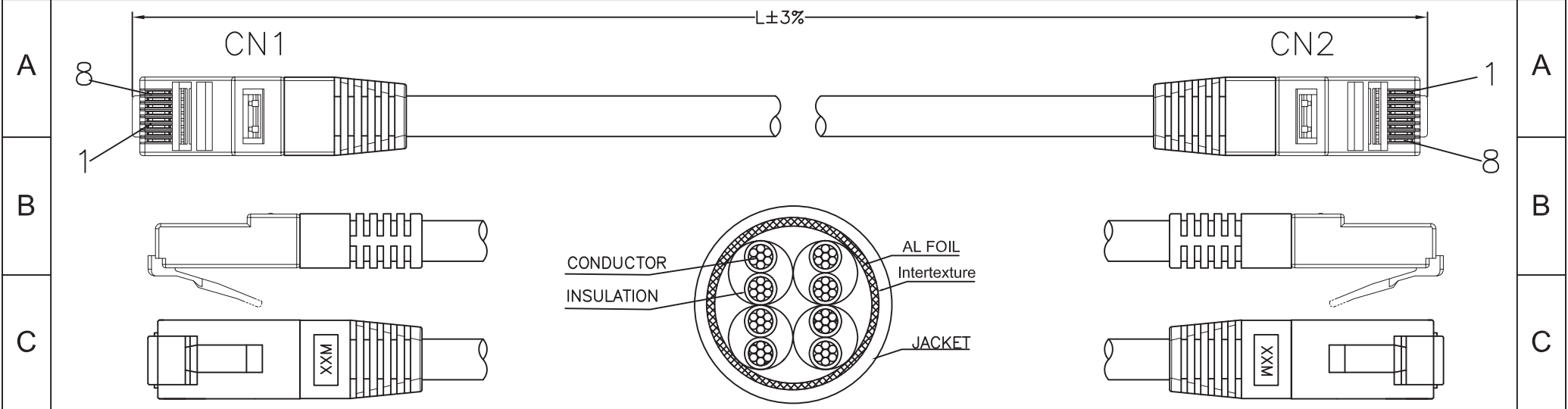
PIN OUT
