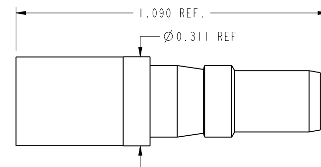
AFTER ASSEMBLY DIMENSIONS SCALE 3.000
