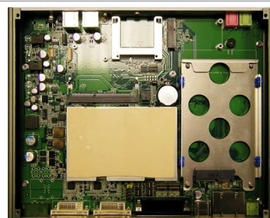
» Fanless Design
