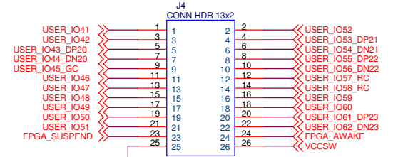
Top side FPGA IO
