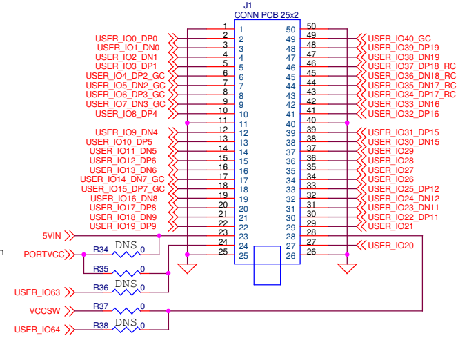
Bottom side FPGA IO (top view)
