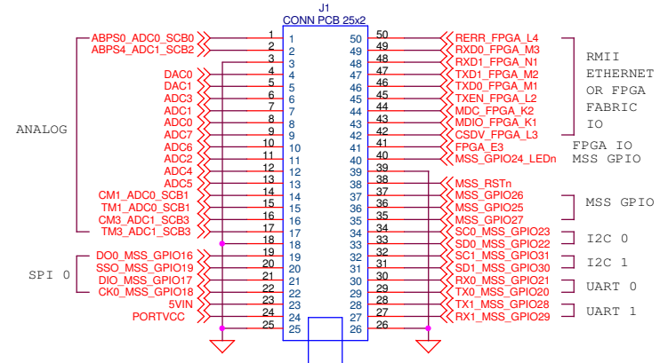
DLP-2232H-SF MODULE IO (top view)
