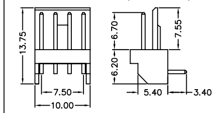
743-72-04TW12 (with wall)
