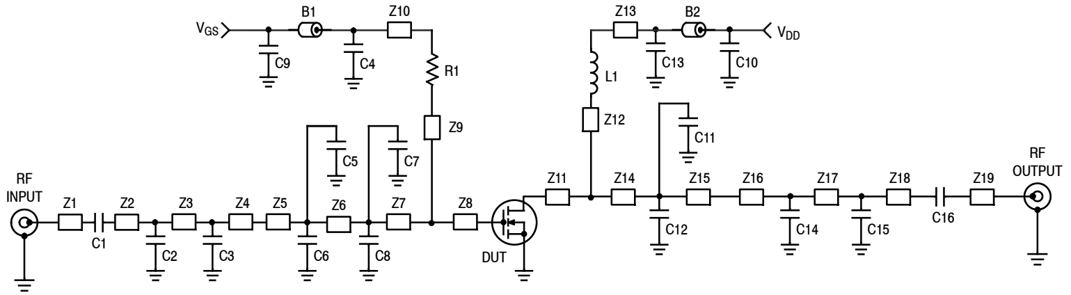
Figure 10. AFT09MS015NT1 UHF Broadband Reference Circuit Schematic — 760-870 MHz
