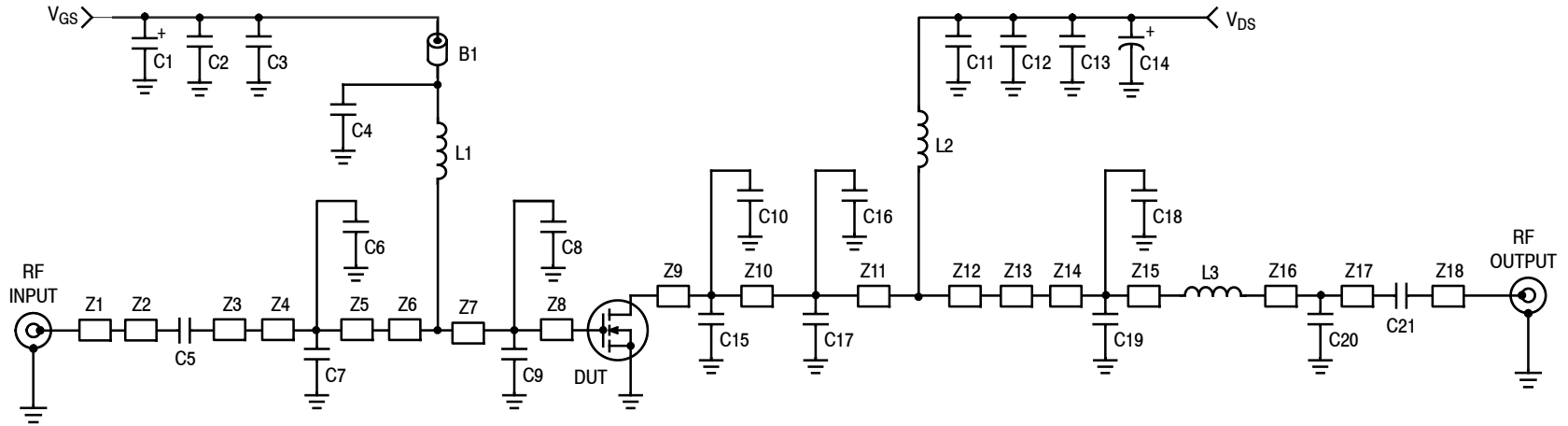
Figure 5. AFT09MS015NT1 Narrowband Test Circuit Schematic — 870 MHz
