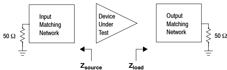
Figure 8. Narrowband Series Equivalent Source and Load Impedance — 870 MHz
