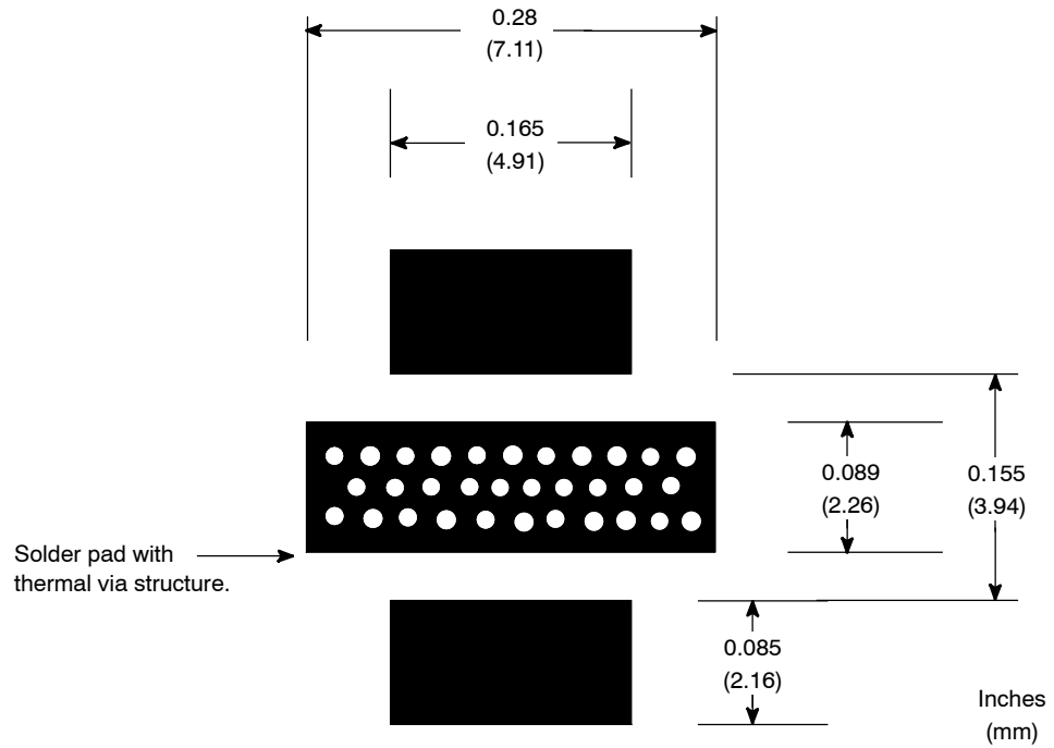
Figure 15. PCB Pad Layout for PLD-1.5W
