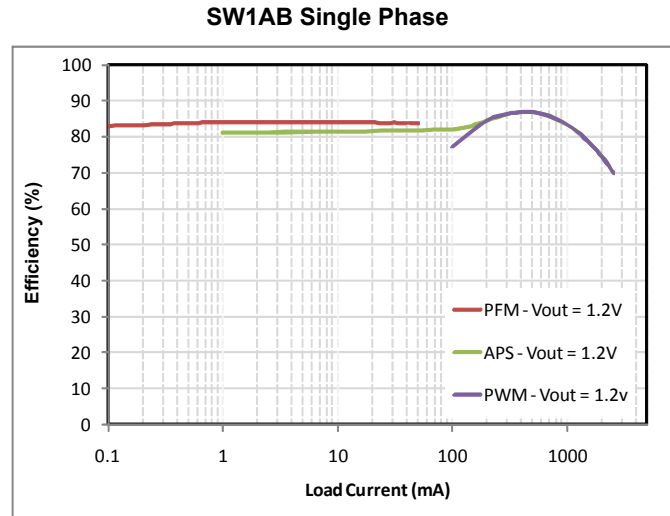
Figure 12. SW1AB Efficiency Waveforms
