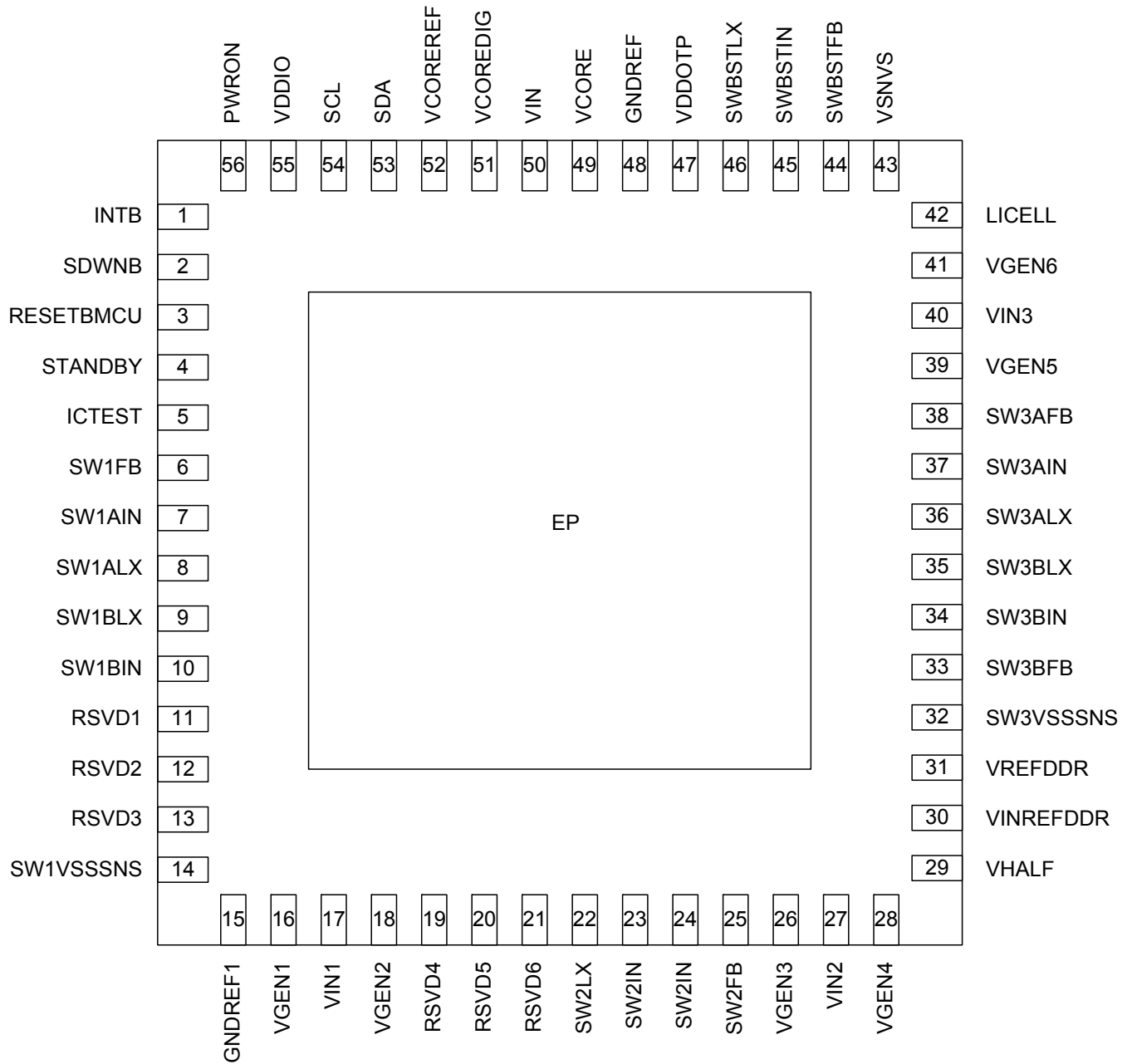
Figure 3. Pinout Diagram
