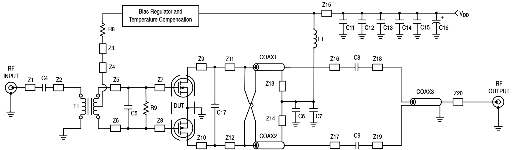
Figure 14. MMRF1316NR1 Broadband Reference Circuit Schematic — 87.5–108 MHz
