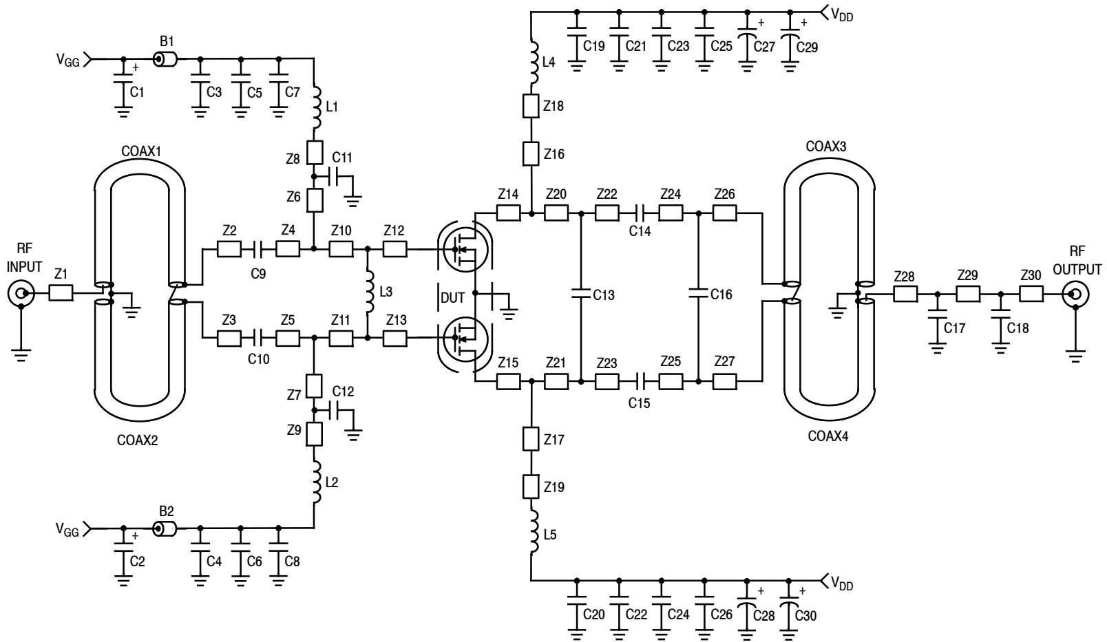
Figure 6. MMRF1316NR1 Narrowband Test Circuit Schematic — 230 MHz
