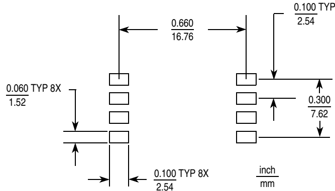
Figure 5. SOP Footprint
