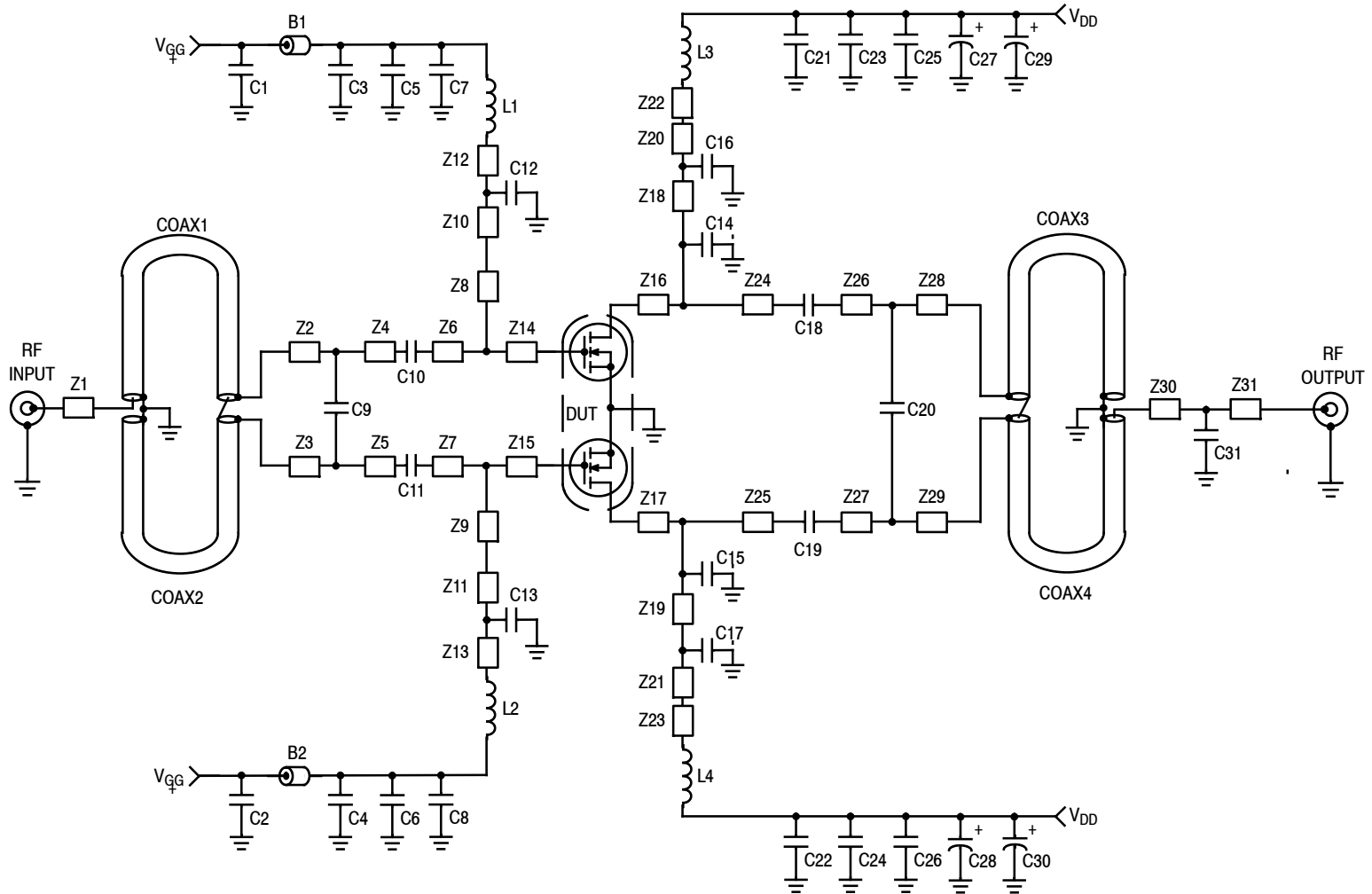
Figure 6. MRFE6VP5150NR1 Narrowband Test Circuit Schematic — 230 MHz
