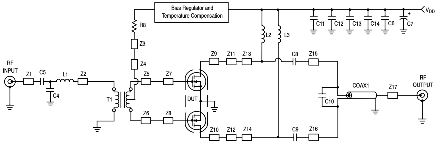
Figure 14. MRFE6VP5150NR1 Broadband Reference Circuit Schematic — 87.5–108 MHz
