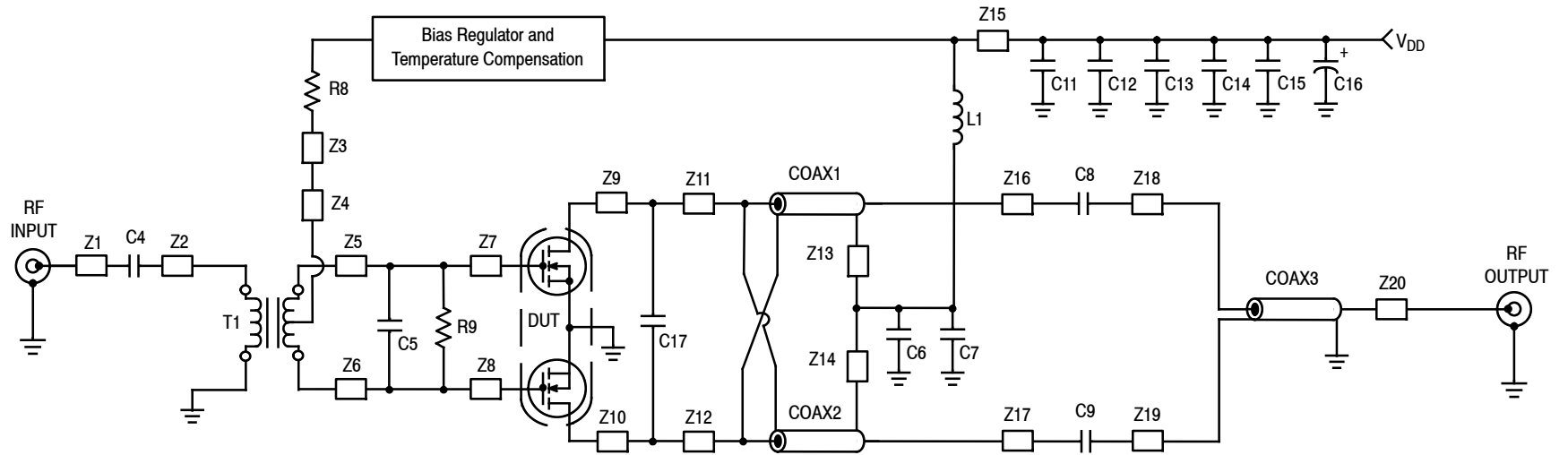
Figure 14. MRFE6VP5300NR1 Broadband Reference Circuit Schematic — 87.5–108 MHz
