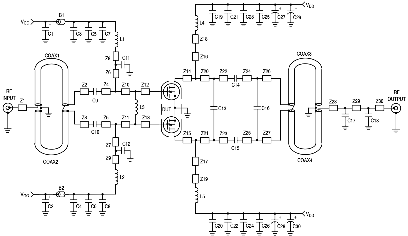
Figure 6. MRFE6VP5300NR1 Narrowband Test Circuit Schematic — 230 MHz
