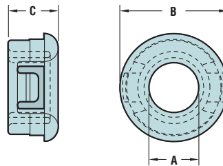
Smooth Bore Bushing
