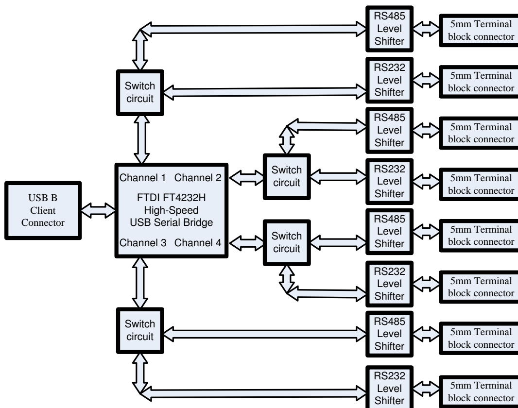
Figure 1.2 USB2-H-9004-M Block Diagram
