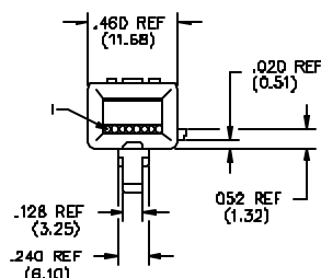
8 CIRCUIT PLUG 1001-8P8C
