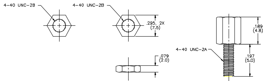
4.8mm x 5mm Female screwlock with nuts
