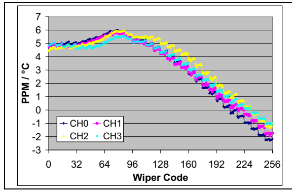
FIGURE 2-59: 50 kΩ – R_{WB} PPM/°C vs. Wiper Setting. ( R_{BW(\text{code}=n, 125^\circ\text{C})}-R_{BW(\text{code}=n, -40^\circ\text{C})})/R_{BW(\text{code}=256, 25^\circ\text{C})}/165^\circ\text{C} * 1,000,000 ) ( V_{DD} = 5.5\text{V} , I_W = 90\ \mu\text{A} ).
