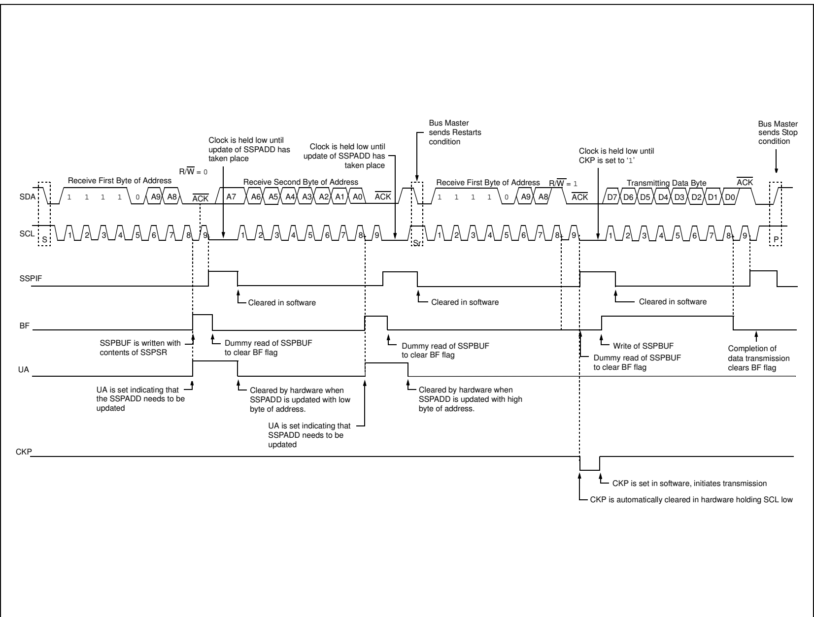
FIGURE 17-13: I 2 C SLAVE MODE TIMING (TRANSMISSION 10-BIT ADDRESS)
