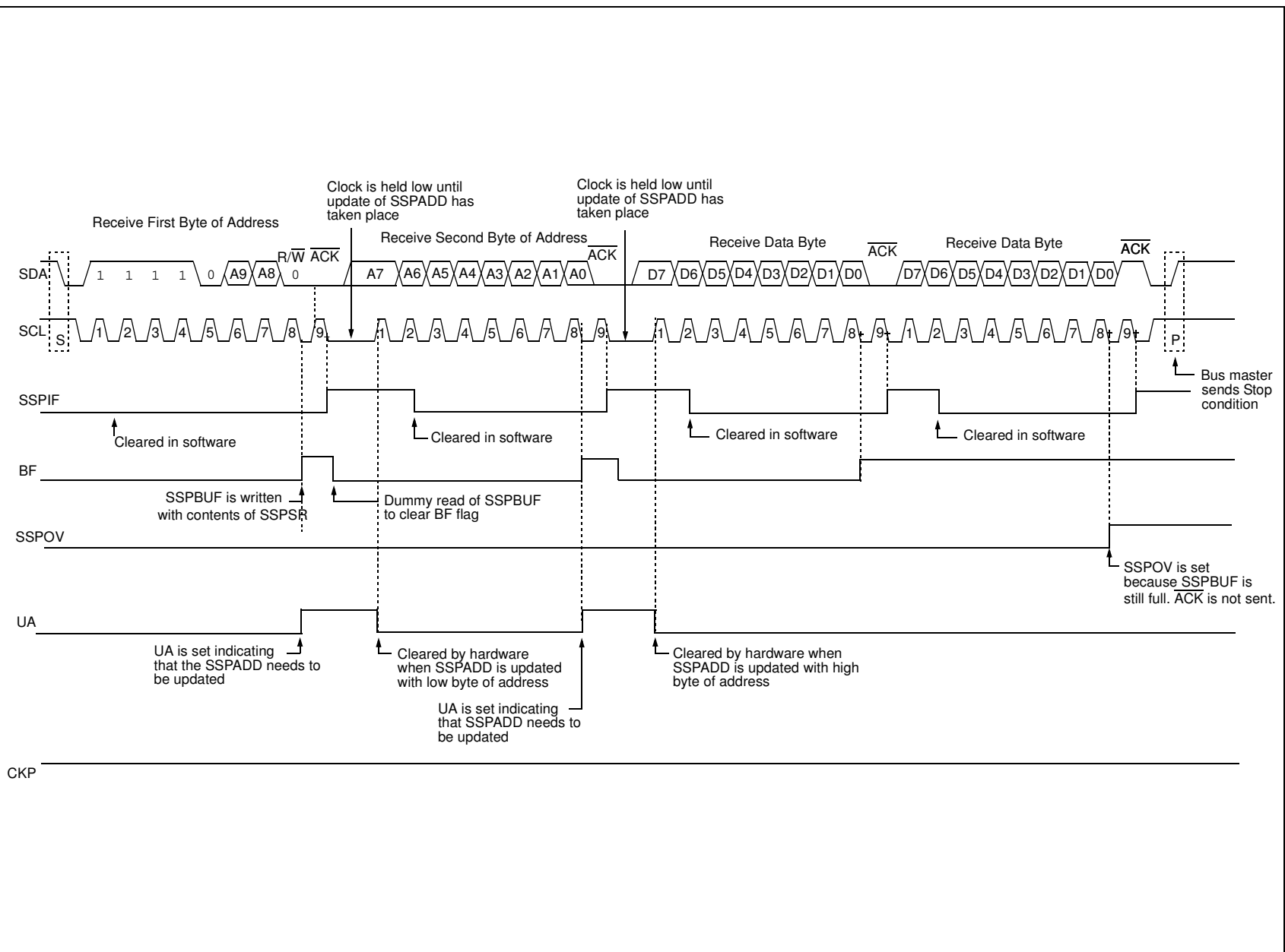
FIGURE 17-11: I 2 C™ SLAVE MODE TIMING (RECEPTION, 10-BIT ADDRESS)
