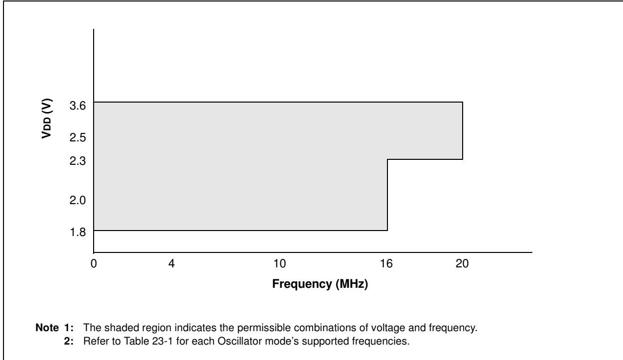
FIGURE 23-5: PIC16LF72X VOLTAGE FREQUENCY GRAPH, -40\text{ }^{\circ}\text{C} \leq T_A \leq +125\text{ }^{\circ}\text{C}
