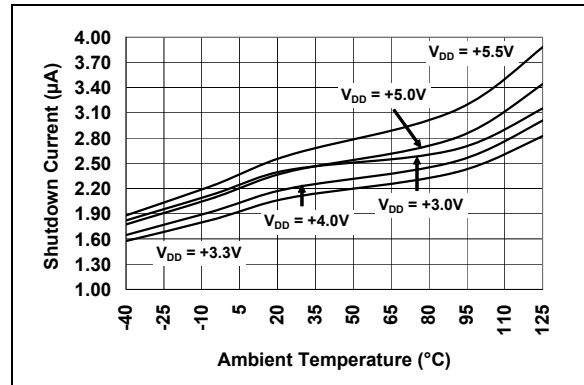
FIGURE 2-4: Shutdown Current vs. Temperature (MCP1631/MCP1631V).
