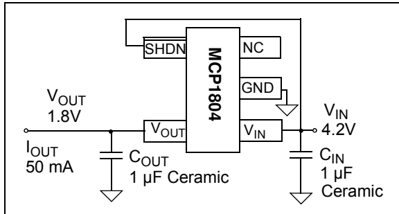
FIGURE 6-1: Typical Application Circuit.
