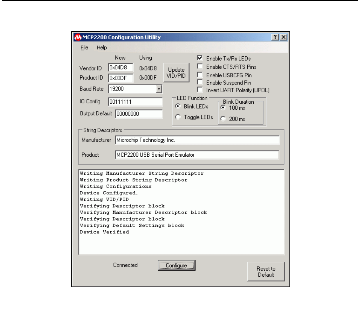
FIGURE 2-1: CONFIGURATION UTILITY
