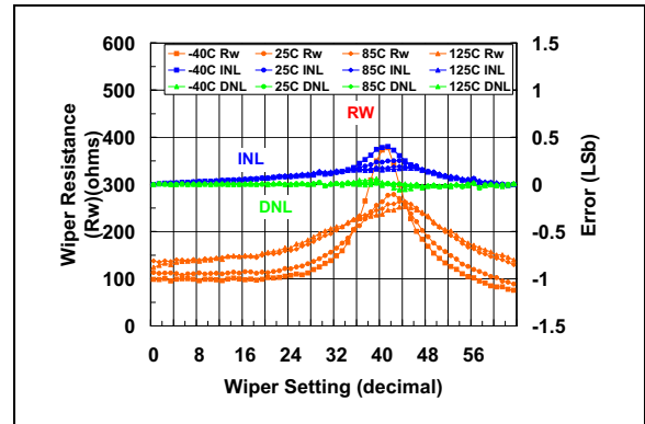
FIGURE 2-40: 50 kΩ Rheo Mode – R_W ( \Omega ), INL (LSb), DNL (LSb) vs. Wiper Setting and Ambient Temperature ( V_{DD} = 2.7\text{V} ).
