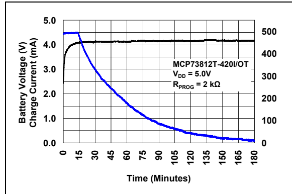
FIGURE 2-21: Typical Charge Profile (950 mAh) Li-Ion Battery.
