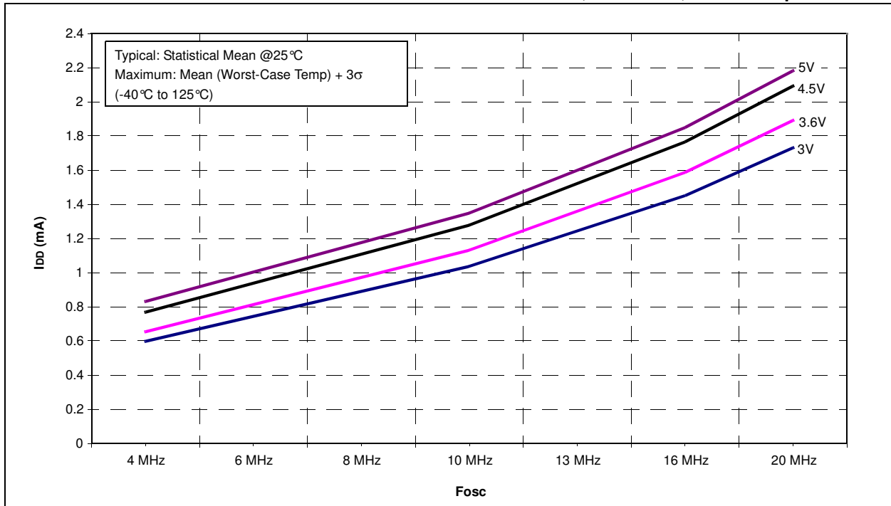
FIGURE 26-9: PIC16F707 MAXIMUM I DD vs. F osc OVER V DD , HS MODE, V CAP = 0.1µF
