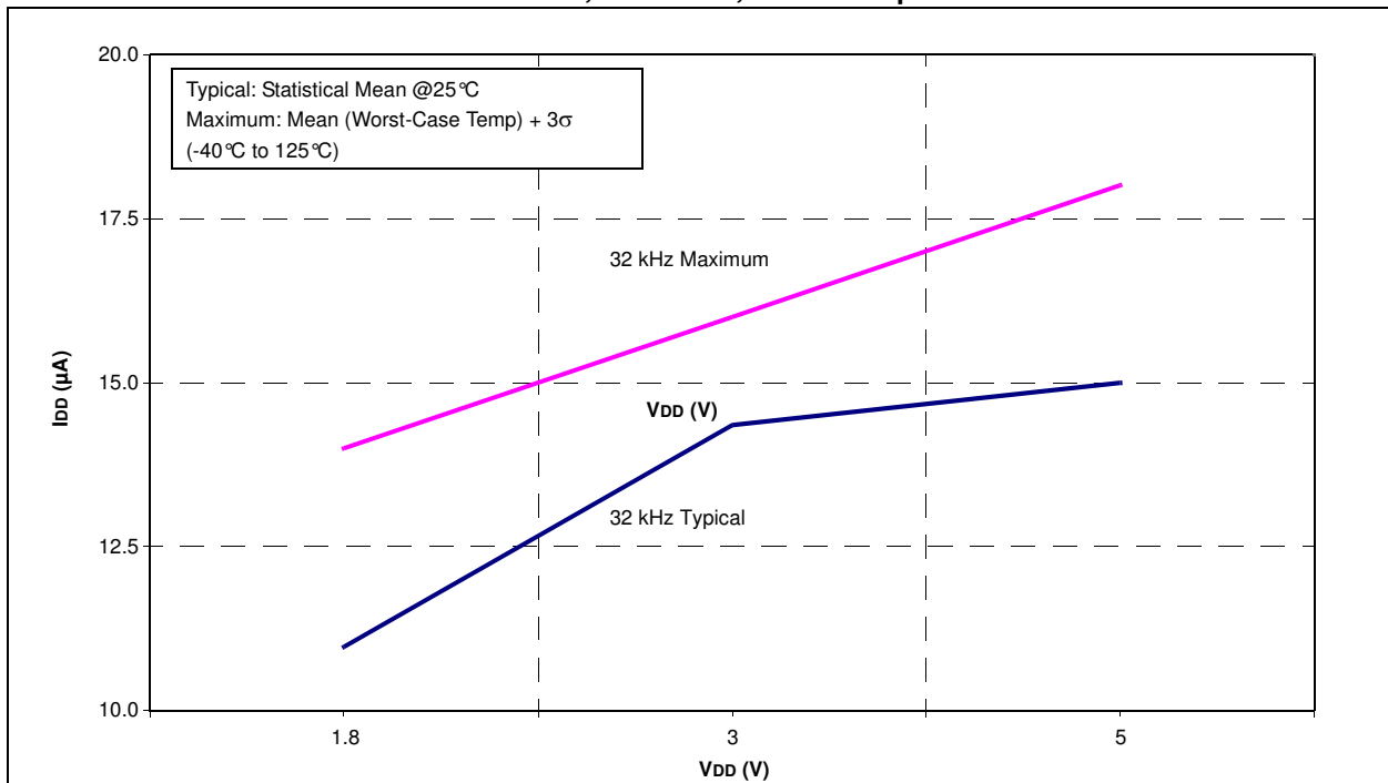
FIGURE 26-17: PIC16F707 I DD vs. V DD , LP MODE, V CAP = 0.1µF
