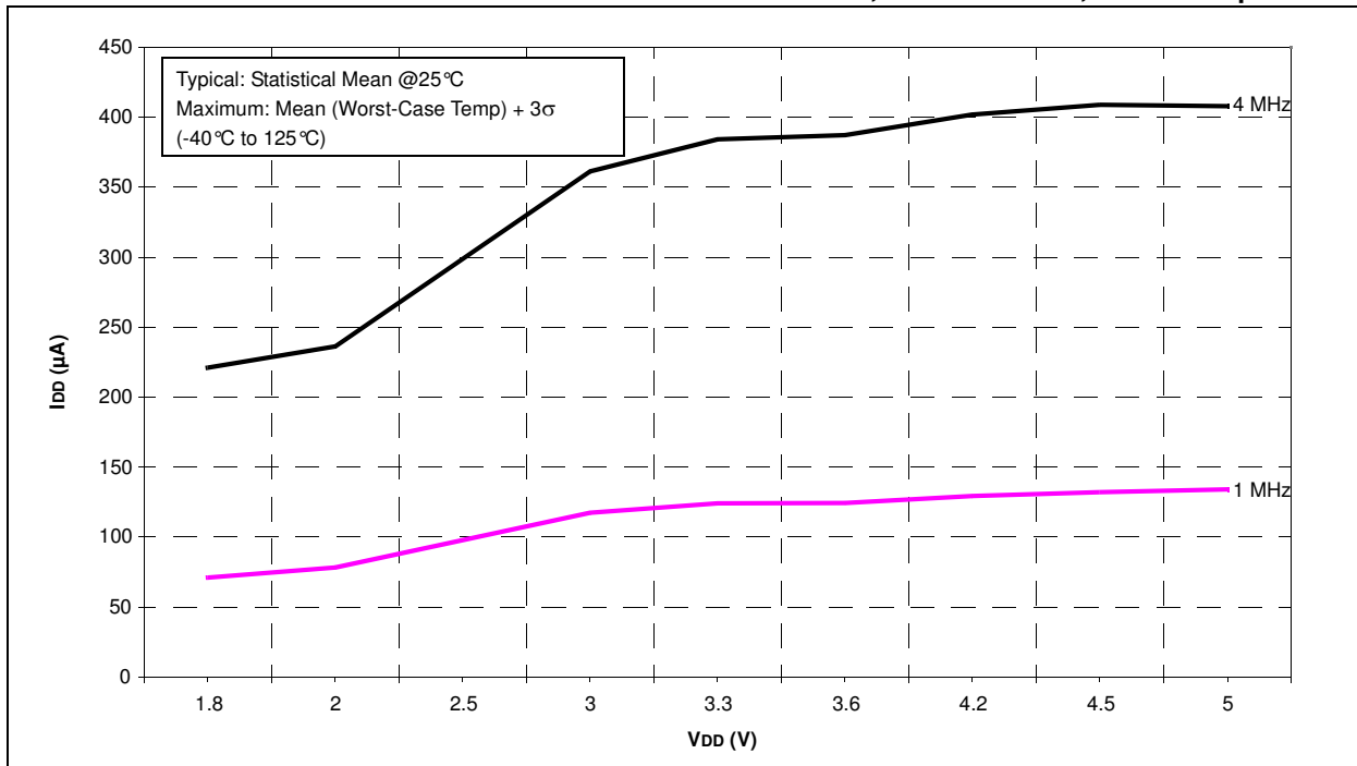
FIGURE 26-7: PIC16F707 TYPICAL I DD vs. V DD OVER F osc , EXTRC MODE, V CAP = 0.1μF
