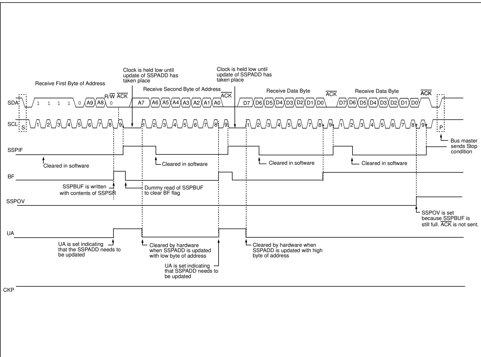
FIGURE 19-11: I 2 C™ SLAVE MODE TIMING (RECEPTION, 10-BIT ADDRESS)
