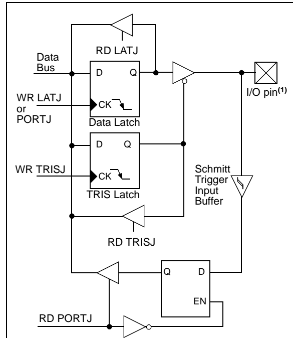
FIGURE 9-19: PORTJ BLOCK DIAGRAM IN I/O MODE
