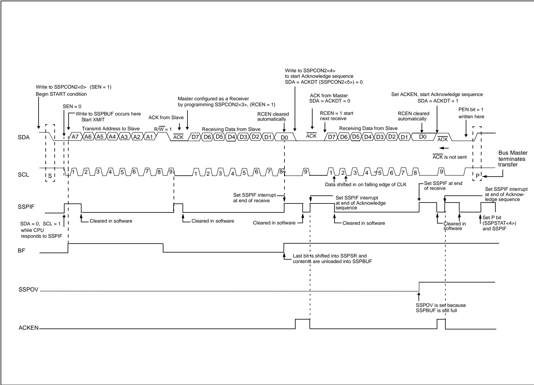
FIGURE 15-16: I 2 C MASTER MODE WAVEFORM (RECEPTION, 7-BIT ADDRESS)
