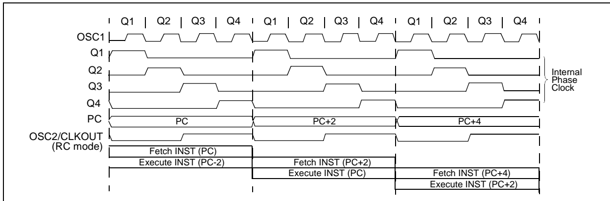
FIGURE 4-6: CLOCK/INSTRUCTION CYCLE
