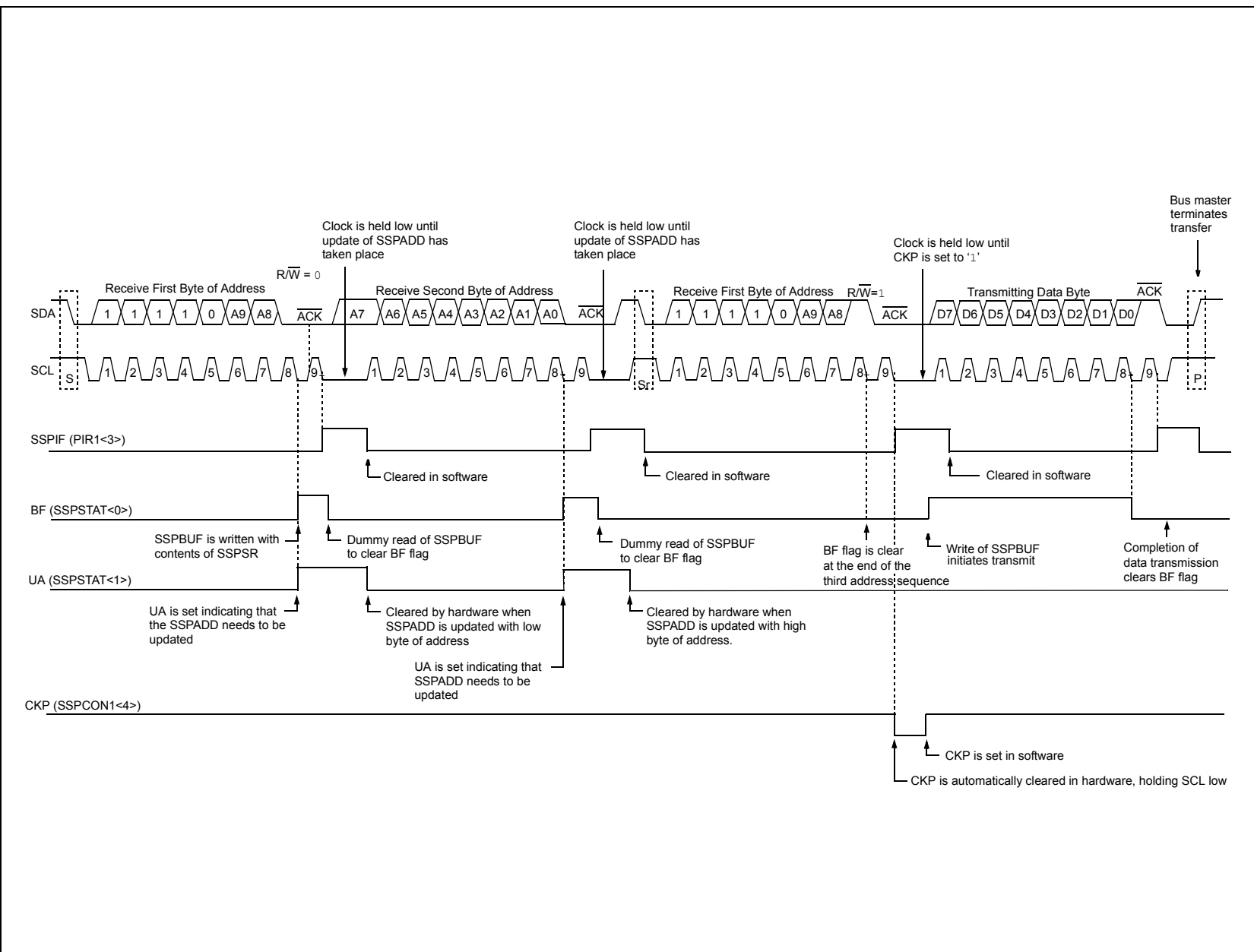
FIGURE 18-13: I 2 C™ SLAVE MODE TIMING (TRANSMISSION, 10-BIT ADDRESSING)
