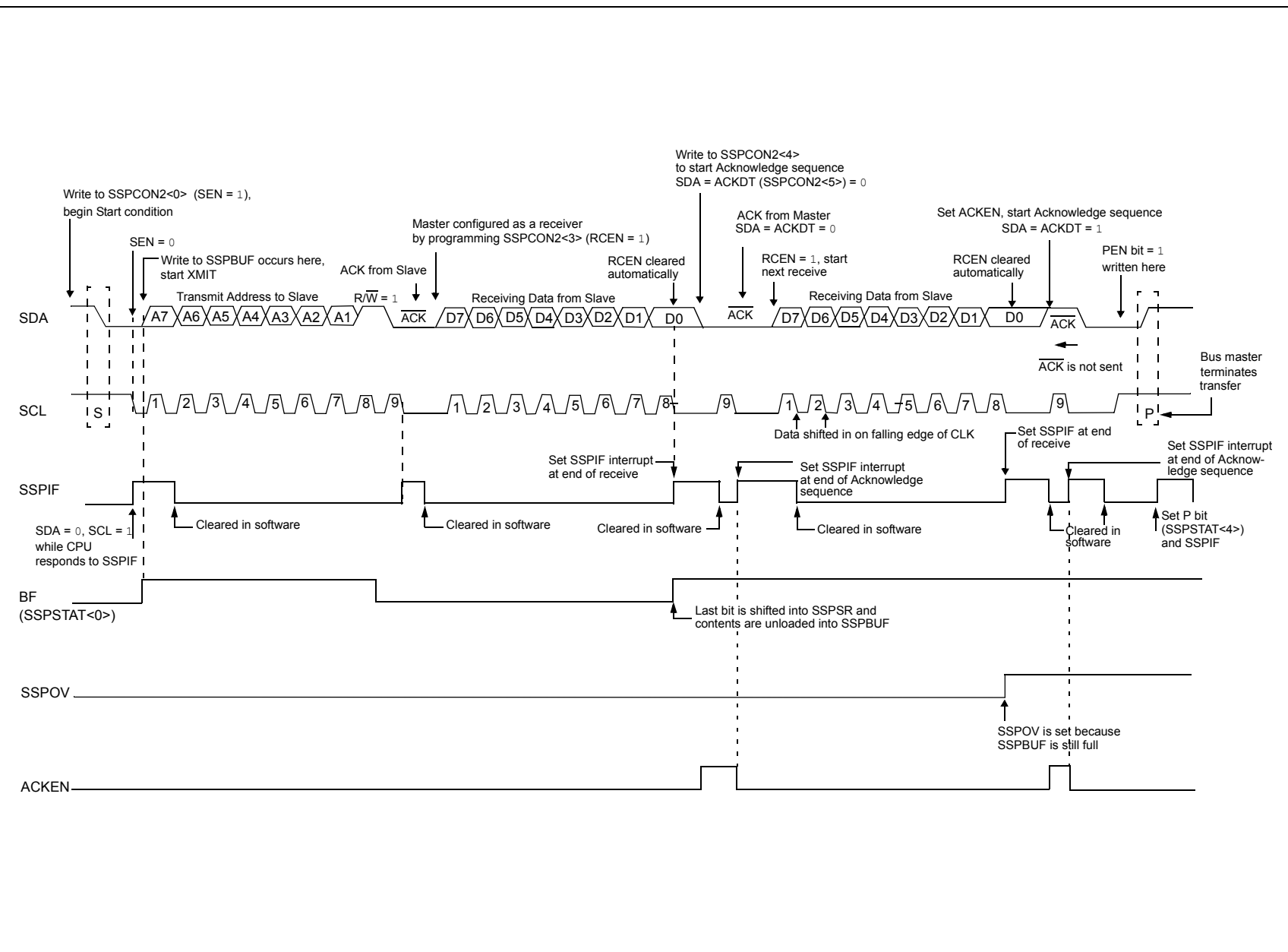
FIGURE 18-24: I 2 C™ MASTER MODE WAVEFORM (RECEPTION, 7-BIT ADDRESSING)
