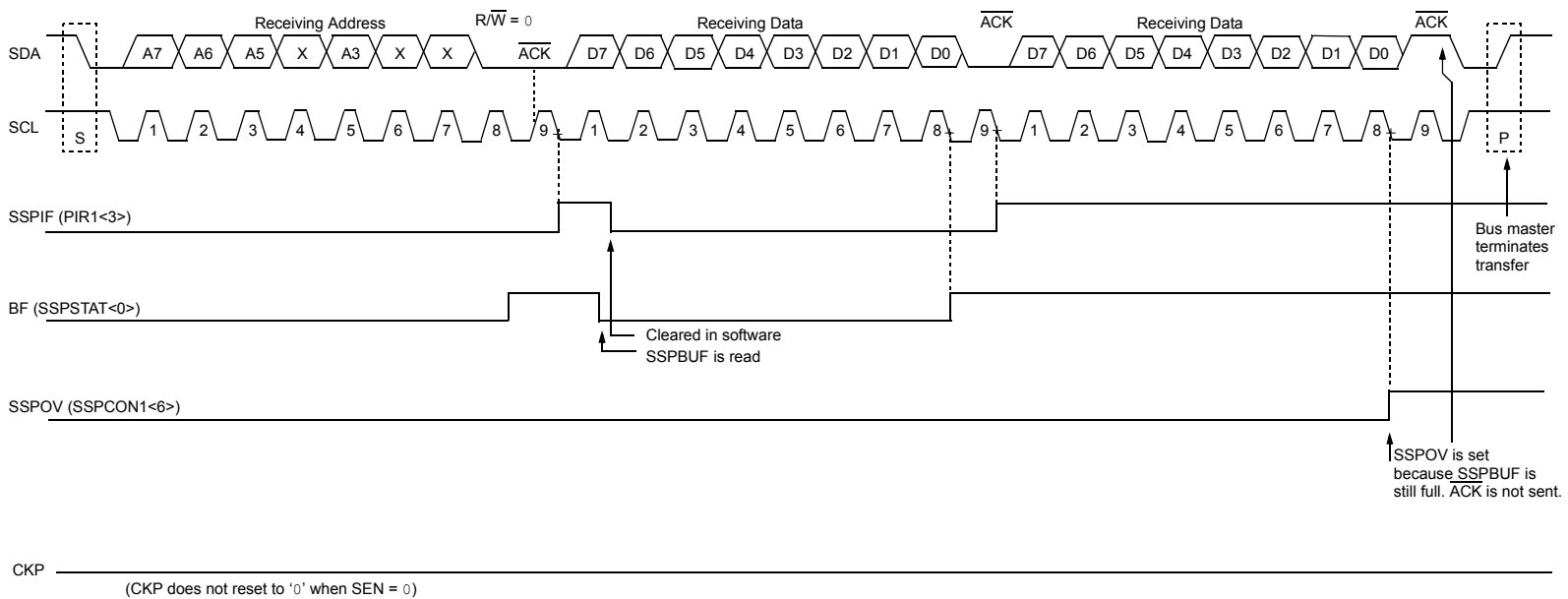
FIGURE 18-9: I 2 C™ SLAVE MODE TIMING WITH SEN = 0 AND ADMASK<5:1> = 01011 (RECEPTION, 7-BIT ADDRESSING)
