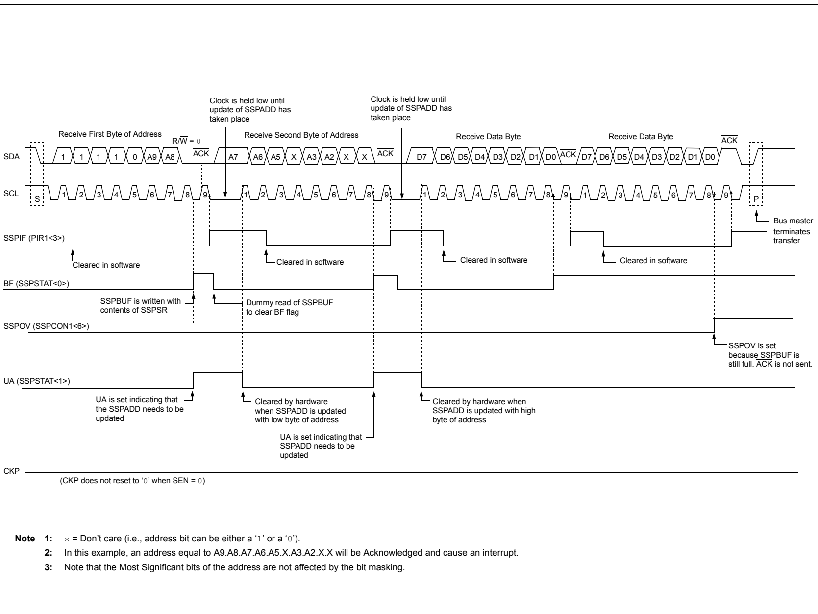
FIGURE 18-11: I 2 C™ SLAVE MODE TIMING WITH SEN = 0 AND ADMSK = 01001 (RECEPTION, 10-BIT ADDRESSING)
