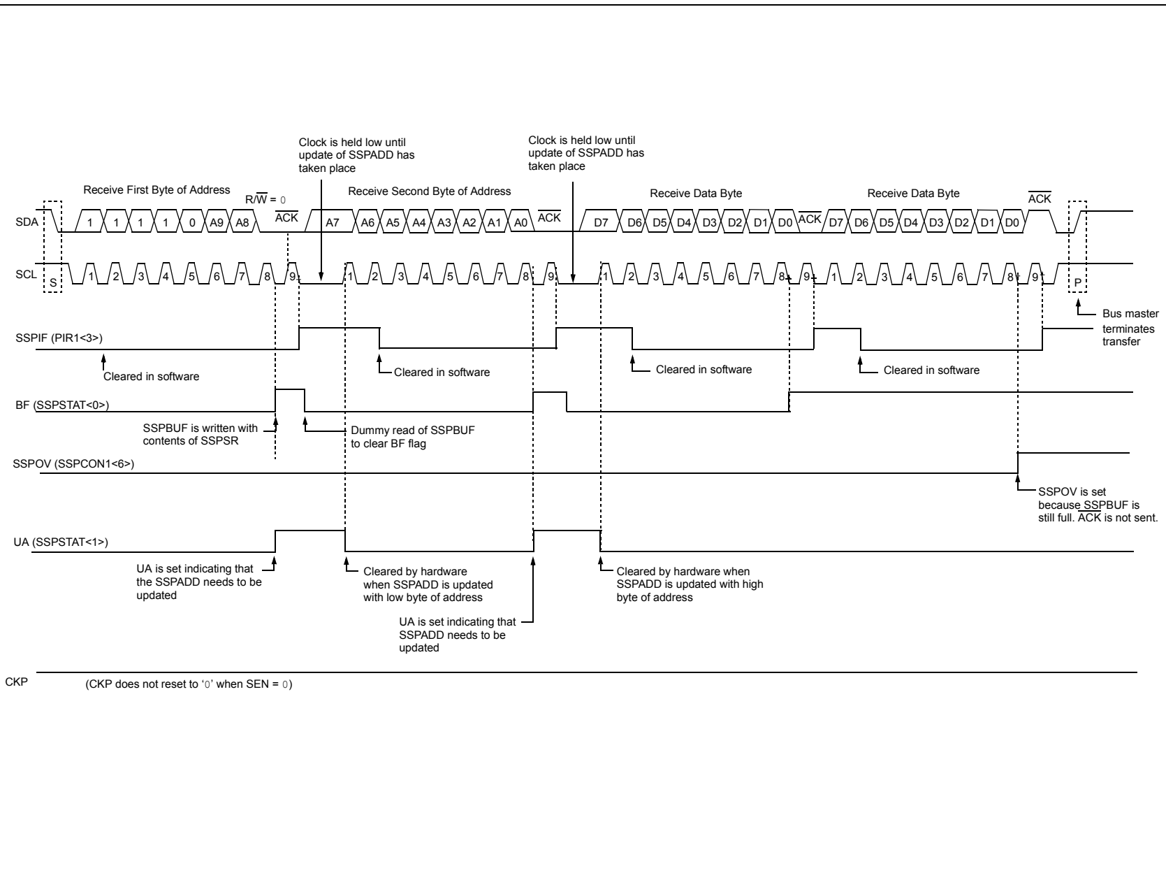
FIGURE 18-12: I 2 C™ SLAVE MODE TIMING WITH SEN = 0 (RECEPTION, 10-BIT ADDRESSING)
