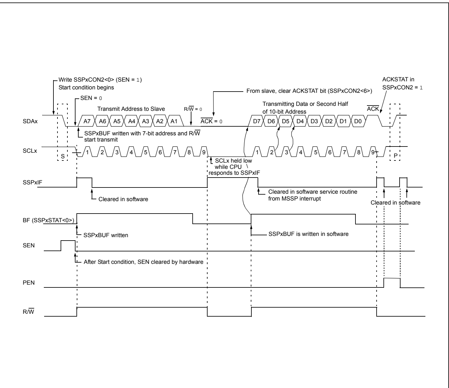
FIGURE 16-21: I 2 C™ MASTER MODE WAVEFORM (TRANSMISSION, 7 OR 10-BIT ADDRESSING)
