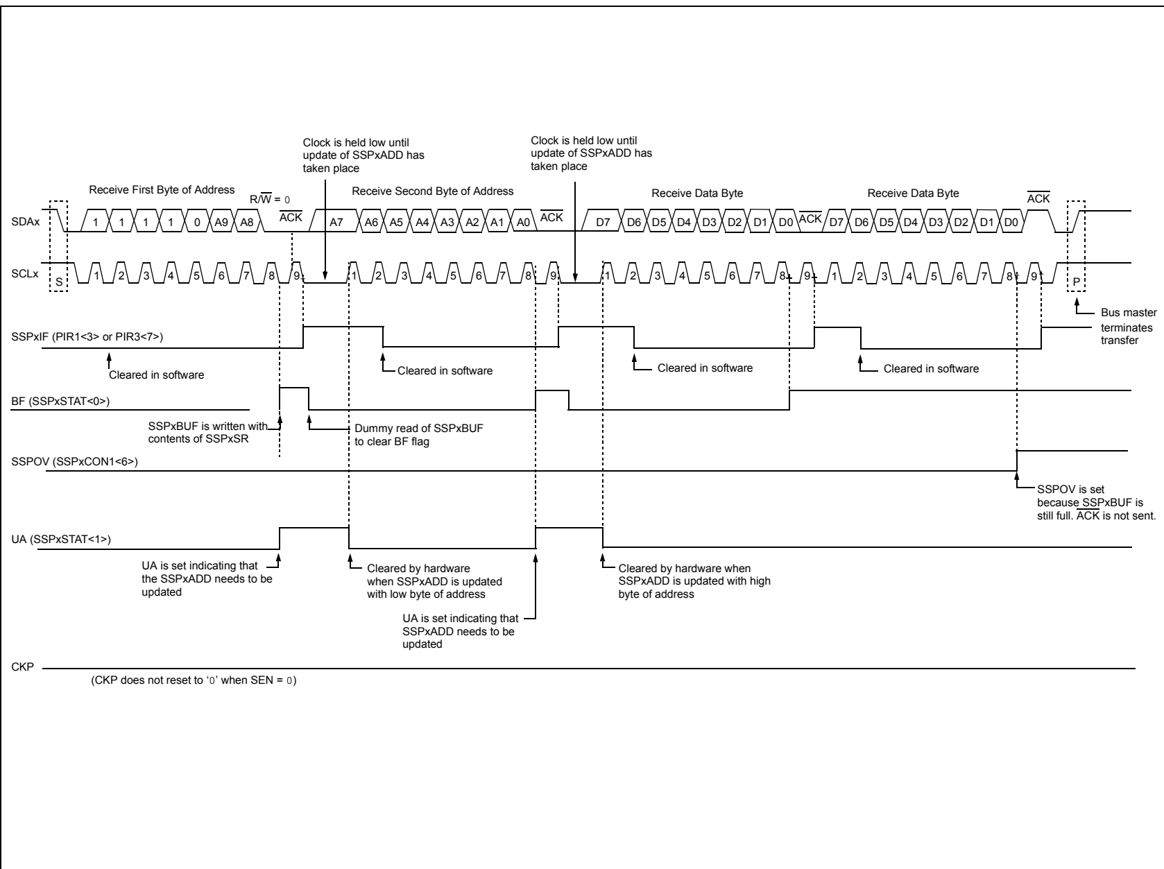
FIGURE 16-10: I 2 C™ SLAVE MODE TIMING WITH SEN = 0 (RECEPTION, 10-BIT ADDRESSING)
