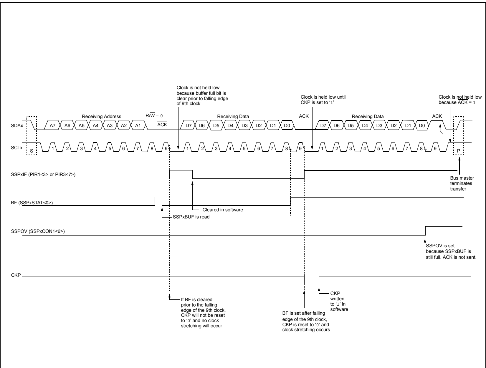
FIGURE 16-13: I 2 C™ SLAVE MODE TIMING WITH SEN = 1 (RECEPTION, 7-BIT ADDRESSING)
