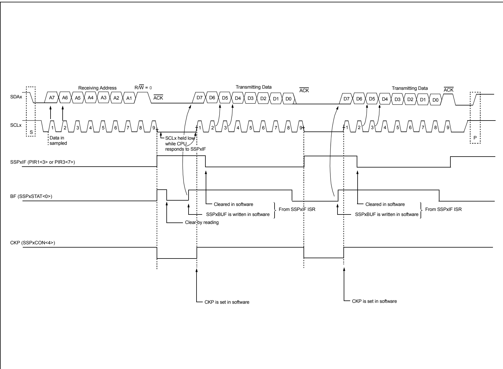
FIGURE 16-9: I 2 C™ SLAVE MODE TIMING (TRANSMISSION, 7-BIT ADDRESSING)
