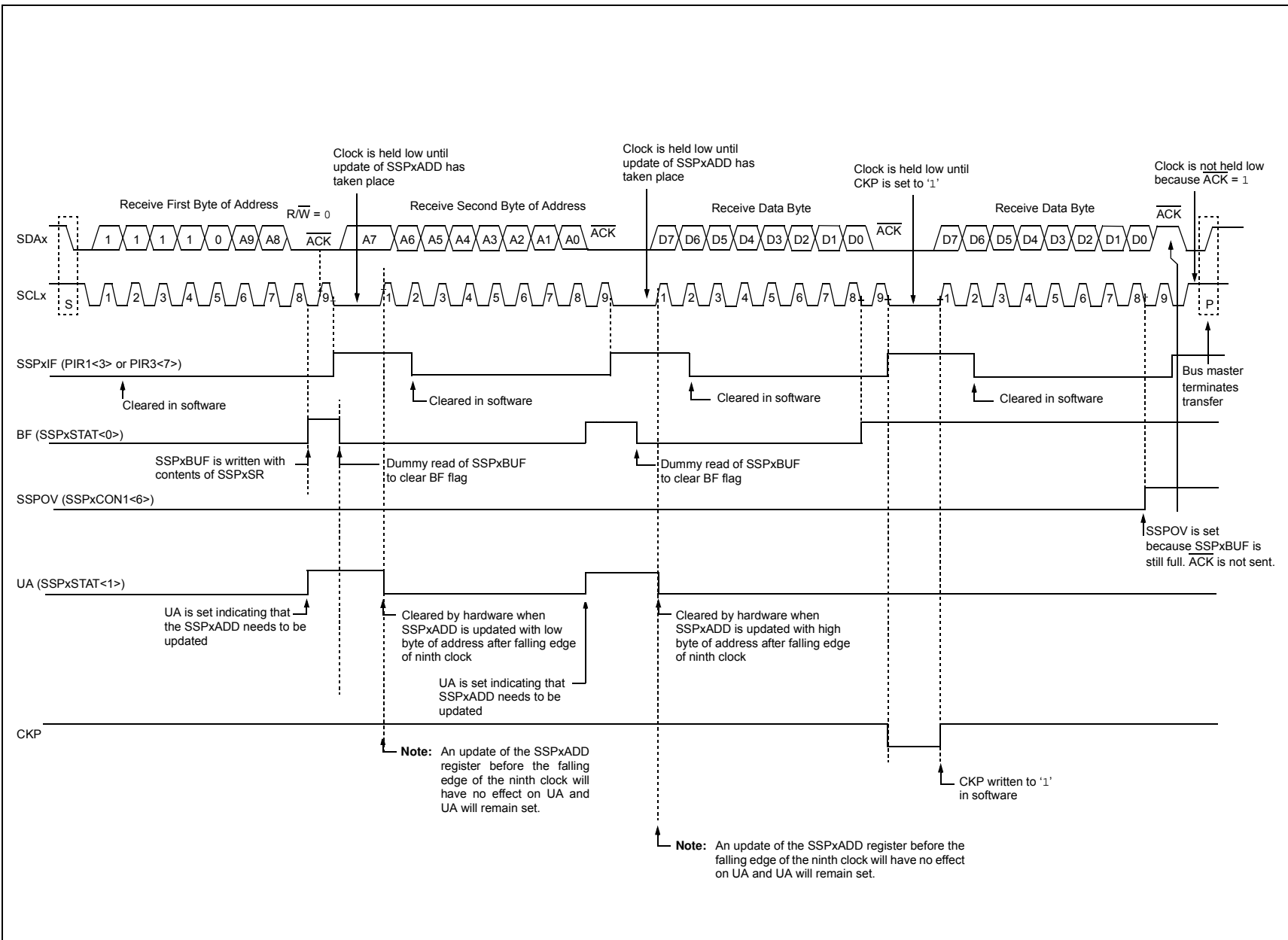
FIGURE 16-14: I 2 C™ SLAVE MODE TIMING WITH SEN = 1 (RECEPTION, 10-BIT ADDRESSING)
