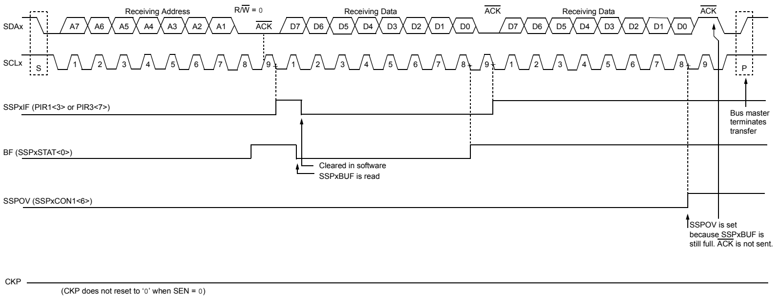
FIGURE 16-8: I 2 C™ SLAVE MODE TIMING WITH SEN = 0 (RECEPTION, 7-BIT ADDRESSING)
