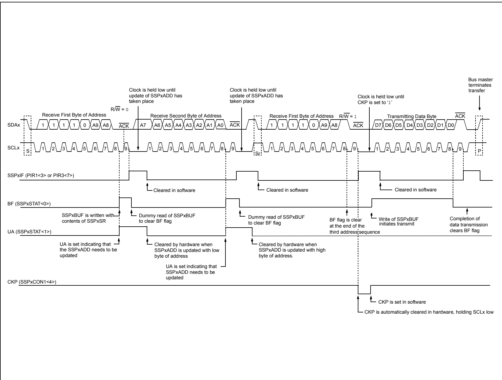
FIGURE 16-11: I 2 C™ SLAVE MODE TIMING (TRANSMISSION, 10-BIT ADDRESSING)
