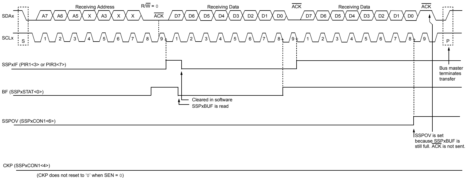
FIGURE 19-9: I 2 C™ SLAVE MODE TIMING WITH SEN = 0 AND ADMSK<5:1> = 01011 (RECEPTION, 7-BIT ADDRESS)
