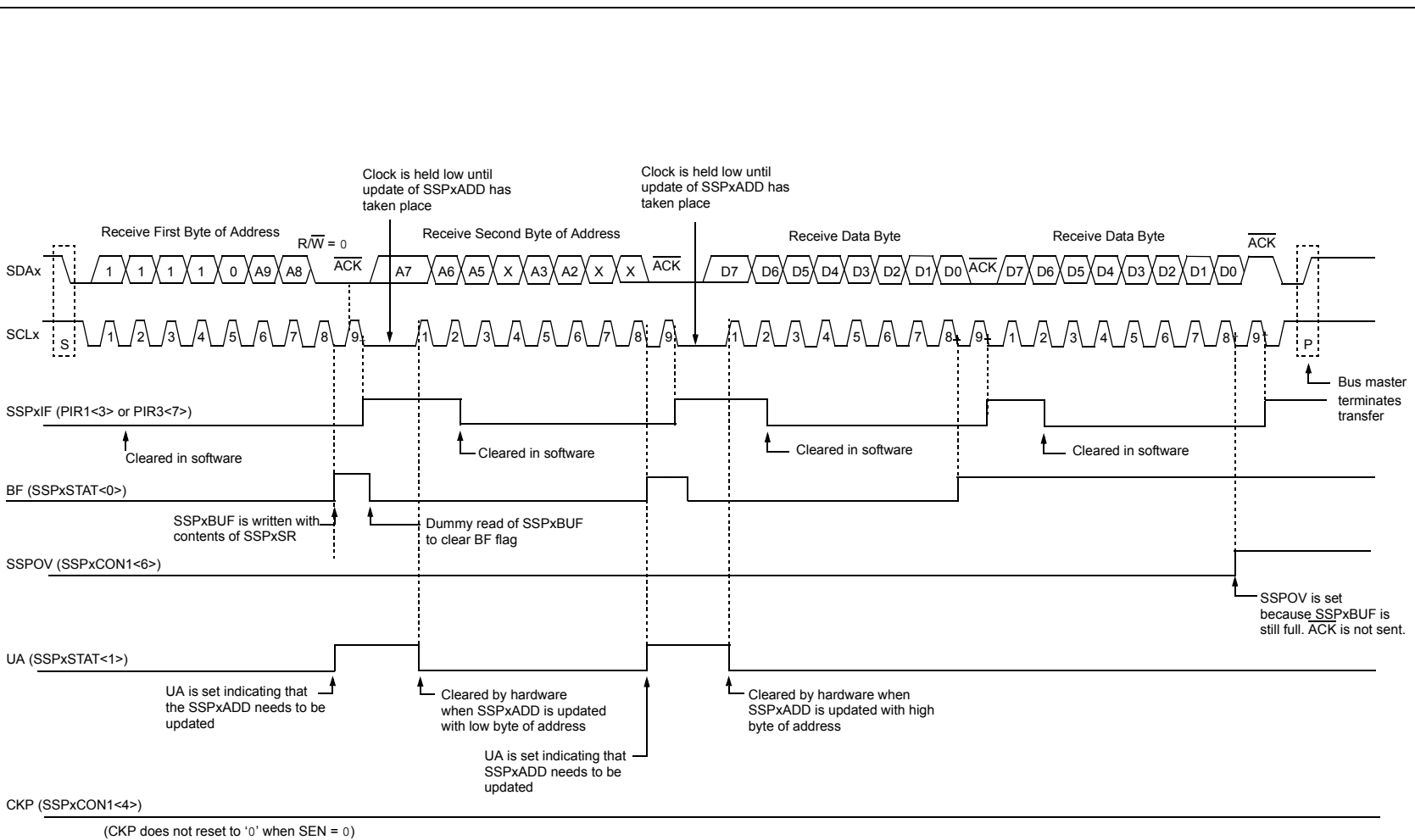
FIGURE 19-11: I 2 C™ SLAVE MODE TIMING WITH SEN = 0 AND ADMASK<5:1> = 01001 (RECEPTION, 10-BIT ADDRESS)
