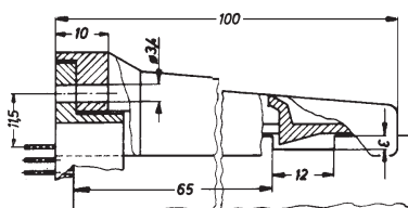
Raster/pitch/pas 3,96 mm
