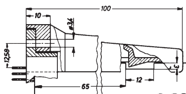
Raster/pitch/pas 5,08 mm
