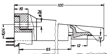
Raster/pitch/pas 2,54 mm
