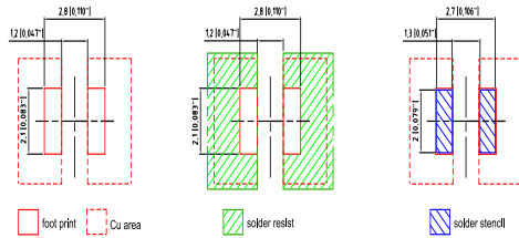
Component Location on Pad
