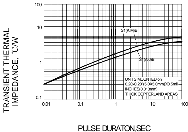
FIG.6-TRANSIENT THERMAL IMPEDANCE
