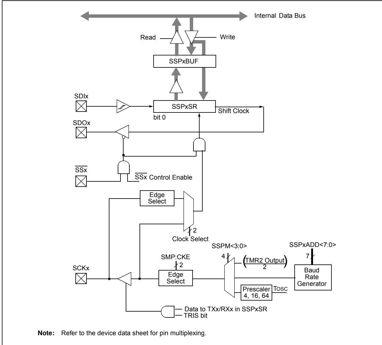
FIGURE 17-1: MSSP BLOCK DIAGRAM (SPI MODE)
