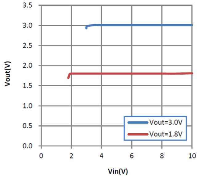
2. Line regulation
