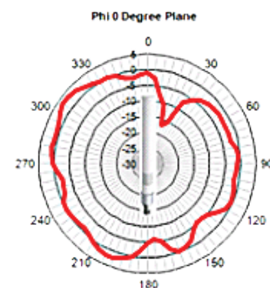
Frequency = 2500 MHz
