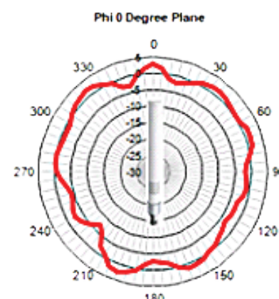
Frequency = 2170 MHz
