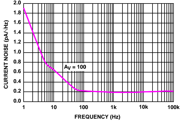
FIGURE 14. EL8172 CURRENT NOISE SPECTRAL DENSITY
