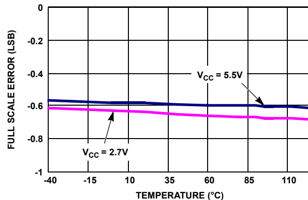
FIGURE 6. FS ERROR vs TEMPERATURE
