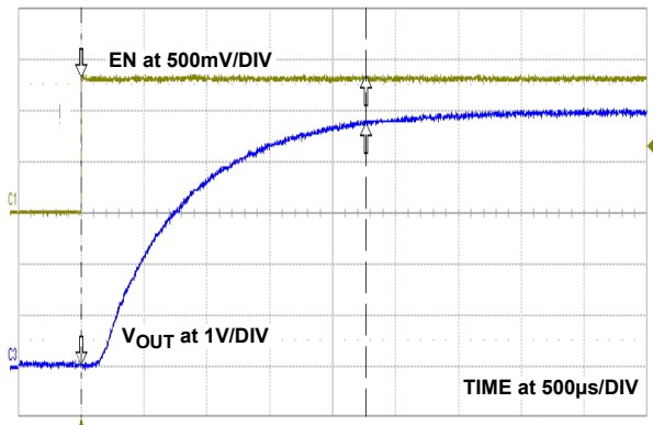
FIGURE 9. START-UP WAVEFORM
