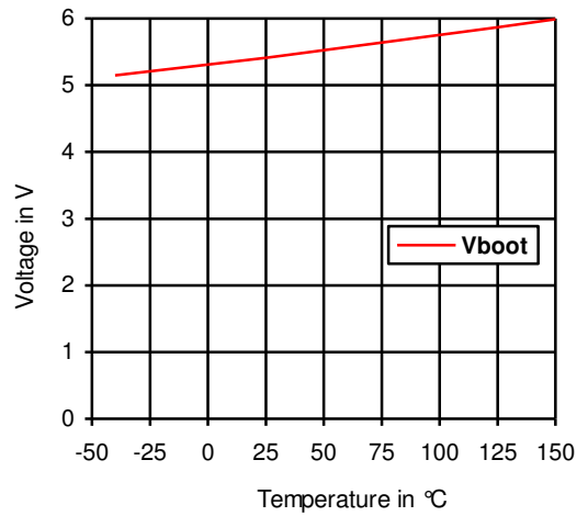
Figure 14: Bootstrap voltage vs. temperature
