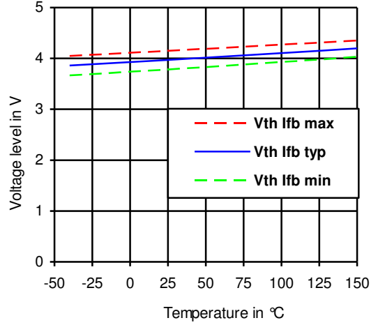
Figure 8: Vth lfb vs. temperature
