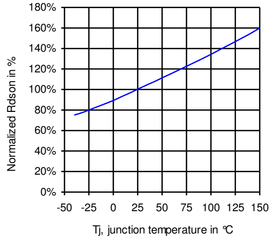
Figure 11: Normalized Rdson Vs Tj
