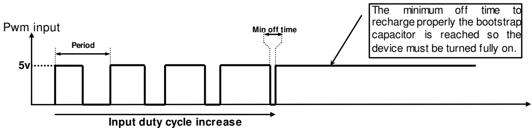
Figure 5: High duty cycle operation recommendation
