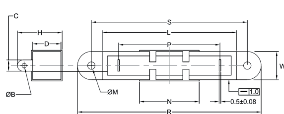
Figure 2 - soldered tag with rugged bracket (SR)
